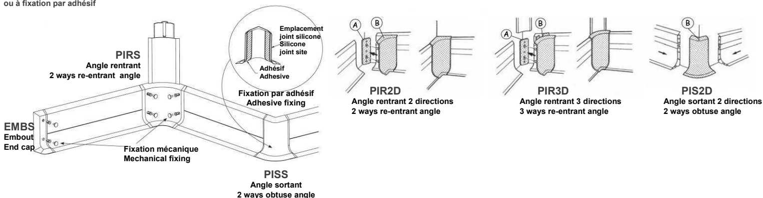
Soft finishing pieces Mechanical or adhesive fastenning
